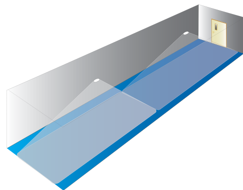
Escape Route (Asymmetric - 1 Lux)
